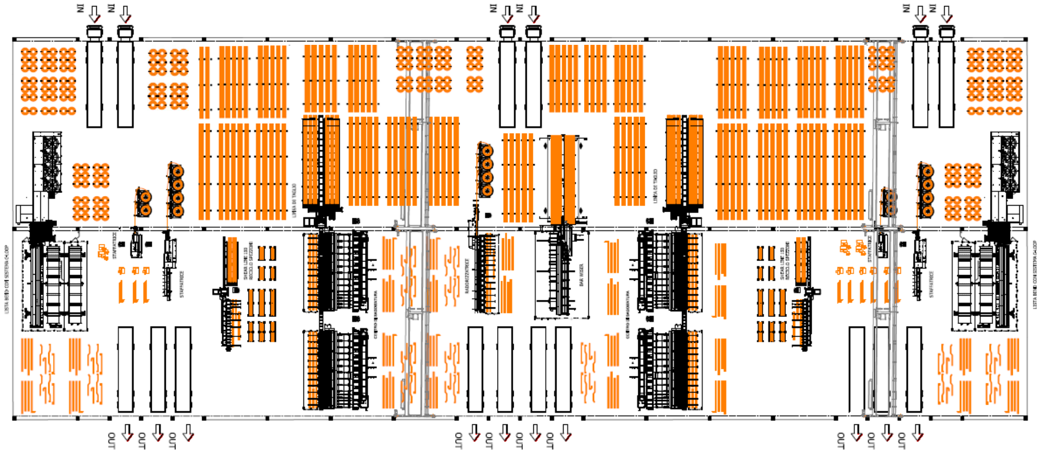
(LAYOUT 5 - 160 m x 30 m a 2 campate)
